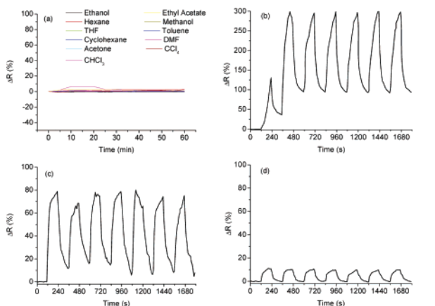
Figure 2. Relative variations of the resistance, \Delta R , for (a) a pure aligned multiwall carbon nanotube array on quartz upon exposure to various chemical vapors, and an aligned carbon nanotube–PVAc film during (b) THF–air cycles, (c) ethanol–air cycles, and (d) cyclohexane–air cycles with time intervals for 2 min “on” and 2 min “off”. \Delta R = (R_{\text{vapor}} - R_0)/R_0 \times 100\% , where R_0 and R_{\text{vapor}} are the resistances of the aligned carbon nanotube–polymer composite film before and after exposure to a chemical vapor, respectively.
